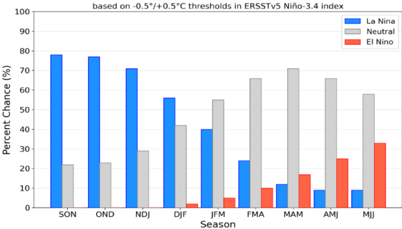
Official NOAA CPC ENSO Probabilities (issued October 2025)
